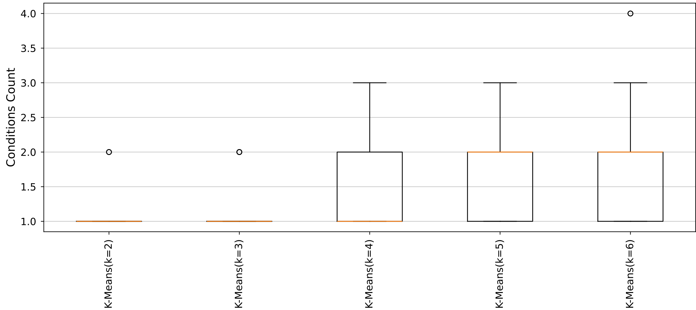
YARA Rules Conditions Count Distribution (Cluster20_Size6 dataset)
